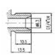
EN16129-H.4-G1/4" LH
